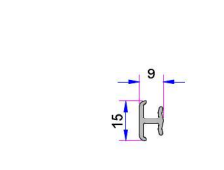
Universal Short Coupling Profile P.A.099.5004.600.0.00.19
