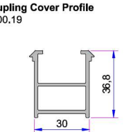
Frame Montage Profile P.A.060.5301.600.0.00.19
