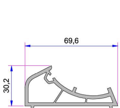
Angled Pipe Profile Adaptor P.A.070.5104.600.0.00.19
