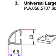
Offset Profile P.A.900.6307.600.0.00.19
