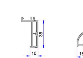
35mm Frame Sill Profile P.A.099.5523.600.0.00.19
