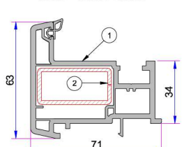
Lap Joint Cover Profile 34012-10140
