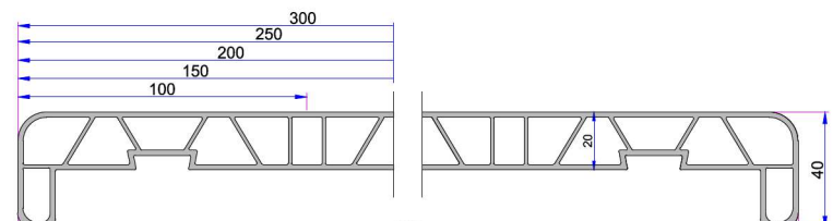
PVC Sill Profile (600mm) P.DNZ.01.60.E.600.19
