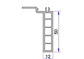
50mm Frame Sill Profile P.A.099.5524.600.0.00.19
