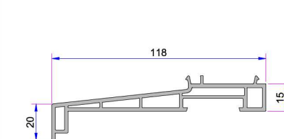
Sill Profile P.A.058.5504.600.0.00.19
