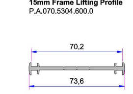
Narrow Coupling Profile P.A.070.5001.600.0.00.19
