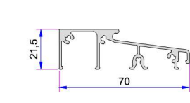
Aluminium Door Threshold Profile AD16-002
