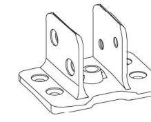
Narrow Mullion Connector P.A.34007-12160
