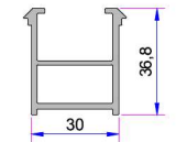
Frame Montage Profile P.A.060.5301.600.0.00.19
