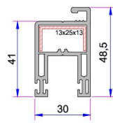
Fly-Screen Sash Profile P.A.242.2305.600.0.00.01
