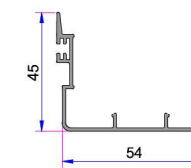
Alm. Sash Cover Profile 16051.601.5.1.1.9016
