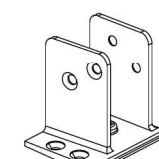
Frame - Frame Connector 34007-14020
