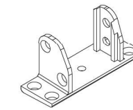
232 Sash Mullion Connector 34007 - 14030
