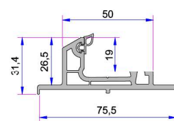
Double Rail Adaptor Profile P.A.232.5800.600.0.00.19
