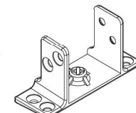
332 Mullion Connector 34007 - 11080
