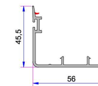
PVC Sash Cover Profile With Seal P.A.232.5700.600.0.00.01
