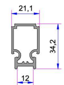
Alm. Double Sash Adaptor 16011.601.5.1.1.9016
