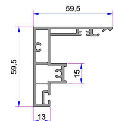
Alm. Sliding Mullion with Three Chambers (In Process)
