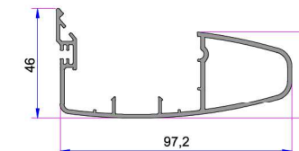
Alm. Sash Cover Grillage Profile 16028.601.5.2.0.9016
