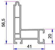
Screen Adaptor Profile P.A.232.5802.600.0.00.19
