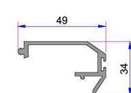
Alm. Cover Profile AD 16 - 013
