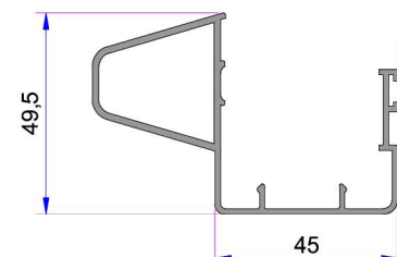
Alm. Sash Cover Grillage Profile (In Process)
