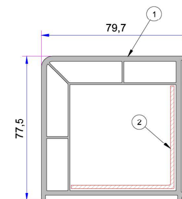
Universal Short Coupling Profile P.A.099.5004.600
