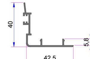
Alm. Sash Cover Profile AD16-031
