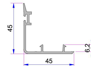
Super Sash Cover Profile P.A.222.5700.600.0.00.19
