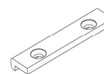
Upper Bedding Piece for Sliding Rail 34009-37010
