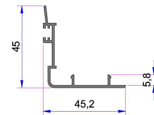
Alm. Super Sash Cover Profile AD16-032
