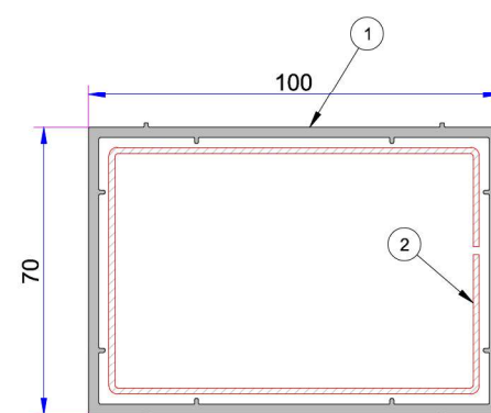
Alm. Double Rail Adaptor AD16-011
