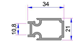
Alm. Double Rail Adaptor AD16-011
