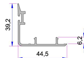
Sash Cover Profile P.A.222.5708.600.0.00.19
