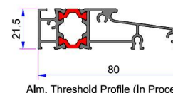
Alm. Threshold Profile (In Process)
