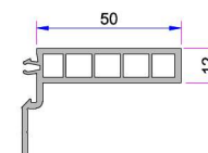
50mm Frame Sill Profile P.A.099.5524.600.0.00.19
