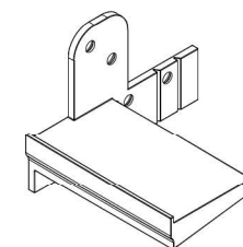
Aluminium Threshold Wedge 221013.0000.L - 221013.0000.R
