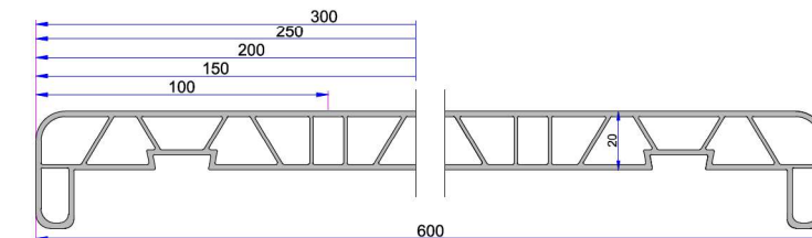
PVC Sill Profile (600mm) P.DNZ.01.60.E.600.19
